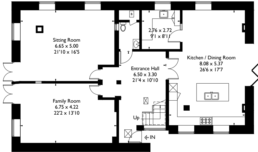
Dairy Ground Floor
