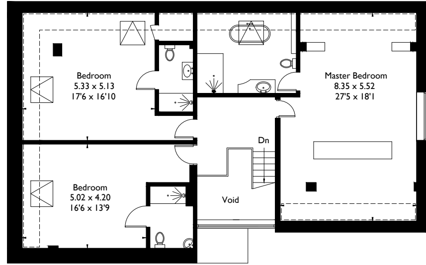
Dairy First Floor
